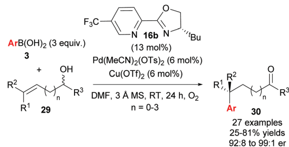
Scheme 20 Enantioselective construction of remote quaternary centres by Sigman and co-workers.
