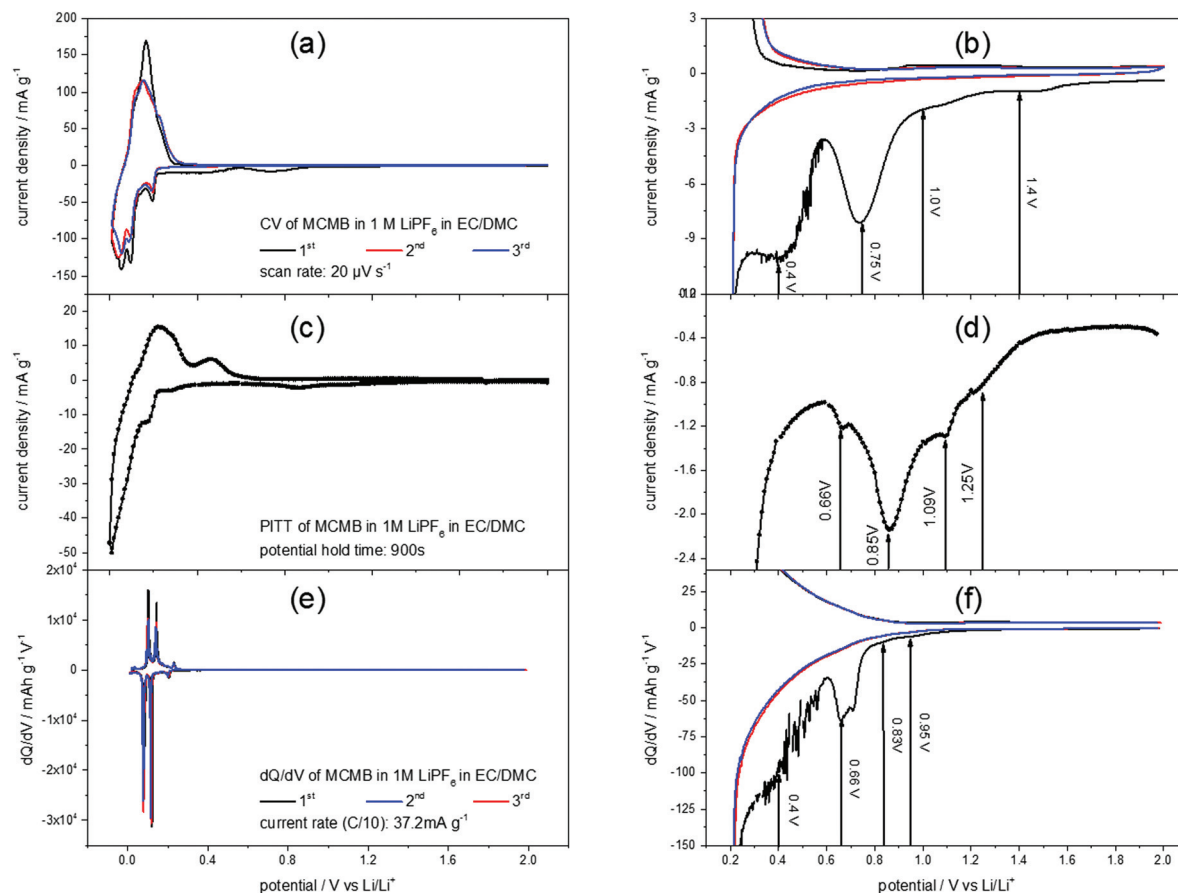
Fig. 2 Voltammograms of MCMB in 1 M \text{LiPF}_6 in EC/DMC (1 : 1) measured by (a and b) cyclic voltammetry (potential sweep rate: 20 \mu\text{V s}^{-1} ) and by (c and d) the potentiostatic intermittent titration technique. For the latter method, the potential was stepwise changed from 2.0 V to 0.01 V and back to 2.0 V in 10 mV steps. After each potential step a current transient was measured for 15 minutes, followed by 15 minutes rest at OCP. The PITT-diagram shows the current density of every transient recorded after 15 minutes at the respective potential. The voltammogram in (e) was derived from a dQ/dV -plot of a charge/discharge curve at a current density of 0.372 \text{ mA g}^{-1} (C/10). (b), (d) and (f) show the magnifications of the CV, PITT and dQ/dV -plot, respectively, in the SEI-formation regime.
