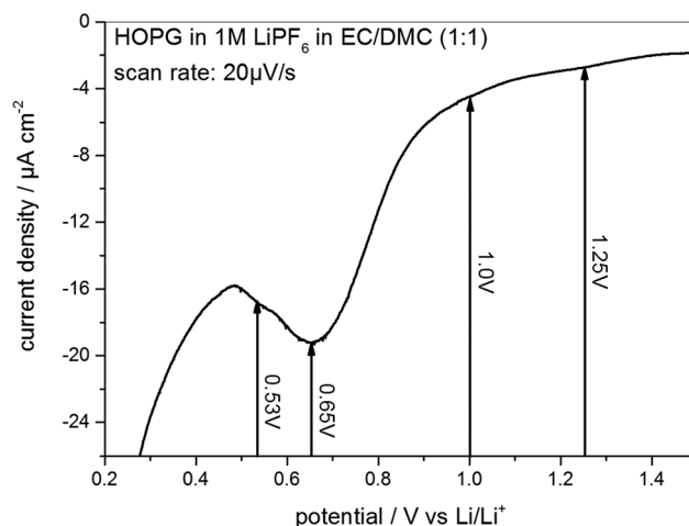
Fig. 3 SEI formation region of a cyclic voltammogram of HOPG in 1 M \text{LiPF}_6 dissolved in EC/DMC (1 : 1). Potential sweep rate: 20 \mu\text{V s}^{-1} .
