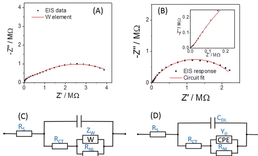
Fig. 5 (A) EIS response at E_{\text{DC}} = +0.240 V (points) and equivalent circuit fit (line) for an r = 25 \mu\text{m} Pt disc electrode in 100 mM aqueous KCl containing 5 mM potassium ferrocyanide. (B) EIS response at E_{\text{DC}} = +0.345 V (points) for an r = 25 \mu\text{m} Pt disc and equivalent circuit fits (lines) in 19 mM added \text{EuCl}_3 in LKE at 703 K. The inset shows an expansion of the higher frequency data, showing the greater than 45^\circ slope consistent with a CPE. (C) The established modified Randles' circuit employed for fitting aqueous disc microelectrode EIS data. (D) The proposed modified Randles' circuit employed for fitting disc MSM EIS data in LKE MS.
