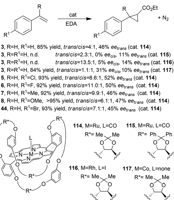
Scheme 21 Synthesis of cyclopropanes 3 , 5–8 and 44 catalysed by 114 , 52 115 , 53 116 53 and 117 . 48
