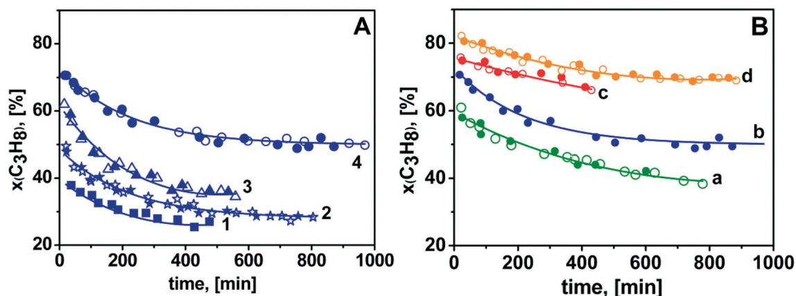
Fig. 6 \text{C}_3\text{H}_8 conversion vs. reaction time during ODH of propane on the Cr/DHS catalysts ( T = 873 K, w = 200 h ^{-1} ) in the as-prepared state (open symbols) and after reaction and subsequent treatment in flowing \text{O}_2 at 873 K for 6 h (full symbols: after 5–8 runs). Panel A refers to the reaction performed using \text{CO}_2 as the oxidant ( \text{C}_3\text{H}_8:\text{CO}_2:\text{N}_2 = 15:30:55 ) on the catalyst: 1) 0.25-Cr/DHS, 2) 0.5-Cr/DHS, 3) 1.0-Cr/DHS, 4) 2.0-Cr/DHS. Panel B shows data obtained on the 2.0-Cr/DHS catalyst under different reaction conditions: a) \text{C}_3\text{H}_8:\text{N}_2 = 15:85 (green curves; full symbols: after 5 runs); b) \text{C}_3\text{H}_8:\text{CO}_2:\text{N}_2 = 15:30:55 (blue curves; full symbols: after 8 runs); c) \text{C}_3\text{H}_8:\text{O}_2:\text{N}_2 = 15:3:82 (red curves; full symbols: after 5 runs); d) \text{C}_3\text{H}_8:\text{CO}_2:\text{O}_2:\text{N}_2 = 15:30:3:52 (orange curves; full symbols: after 8 runs).
