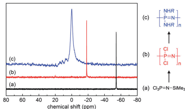
Fig. 4 Sample ^{31}\text{P}\{^1\text{H}\} NMR spectra of the monomer trichlorophosphoranimine \text{Cl}_3\text{PNSiMe}_3 (a), polydichlorophosphazene [\text{NP}(\text{Cl})_2]_n (b) and a macrosubstituted poly(organo)phosphazene [\text{NP}(\text{NHR})_2]_n (c) demonstrating the simple tracking of the reaction progression. Adapted from H. Henke et al. , J. Polym. Sci., Part A: Polym. Chem. , 2013, 51 , 4467. Copyright 2013 Wiley Periodicals, Inc. 12
