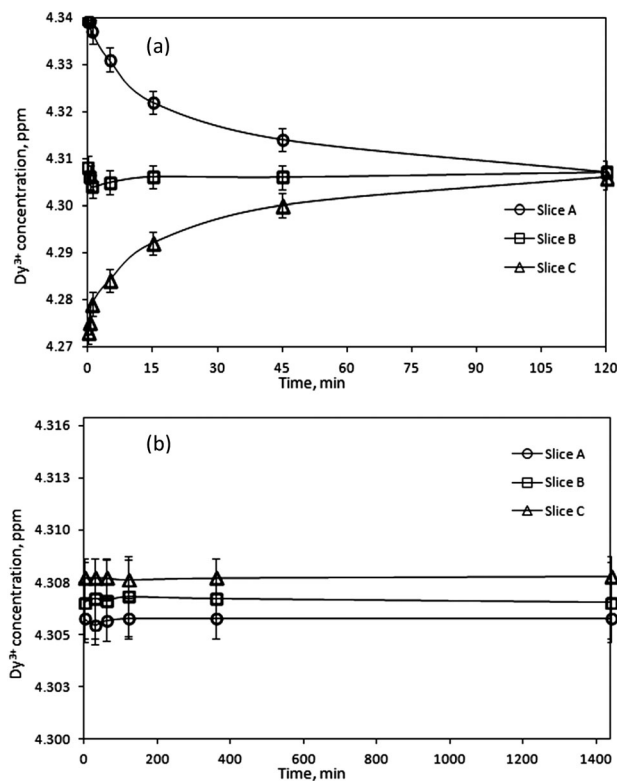
Fig. 5 (a) Concentration changes of \text{Dy}^{3+} ions after removal of the magnetic field gradient (NdFeB permanent magnet, B = 0.5 T, BdB/dz = 14.5 T ^2 m ^{-1} ); (b) reference sample without the presence of a magnetic field. Slices A, B and C are the distances from the strongest magnetic field gradient point: slice A: 0–2 mm, slice B: 2–4 mm and slice C: 4–6 mm.
