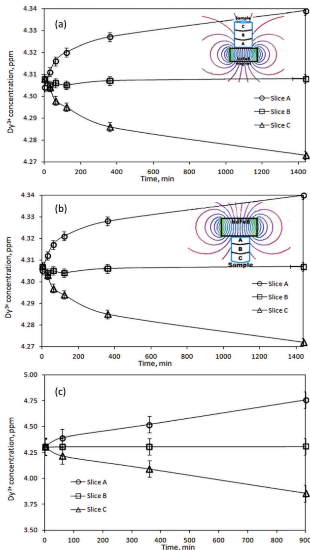
Fig. 2 (a and b) Concentration changes of \text{Dy}^{3+} ions induced by a NdFeB permanent magnet ( B = 0.5 T, BdB/dz = 14.5 T 2 m -1 ), and (c) by a superconducting magnet ( B = 5 T, BdB/dz = 189 T 2 m -1 ) in gel samples. Slices A, B and C are the distances from the strongest magnetic field gradient point: slice A: 0–2 mm, slice B: 2–4 mm and slice C: 4–6 mm.
