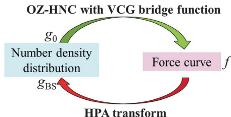
Fig. 2 Closed cycle of the computational validation test. If g_{BS} calculated by using HPA transform fits the benchmark structure g_0 or is similar to g_0 , it indicates that HPA transform is a valid method for estimation of g_0 . In the validation test, OZ-HNC with the VCG bridge function, a highly precise method, is used for the calculation of g_0 and f . (In a practical use, the force curve is prepared by AFM, and the force curve is transformed into the number density distribution through HPA transform.)
