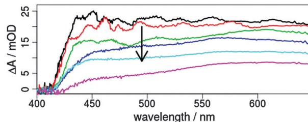
Fig. 4 Transient absorption spectra of the dye-sensitized TiO 2 -layer 2T after 0.5 (black), 1 (red), 3 (green), 10 (blue), 50 (light blue) and 300 ps (magenta) excited at 388 nm with pulses perpendicular polarised to the probe. The observed changes are indicated with an arrow.
