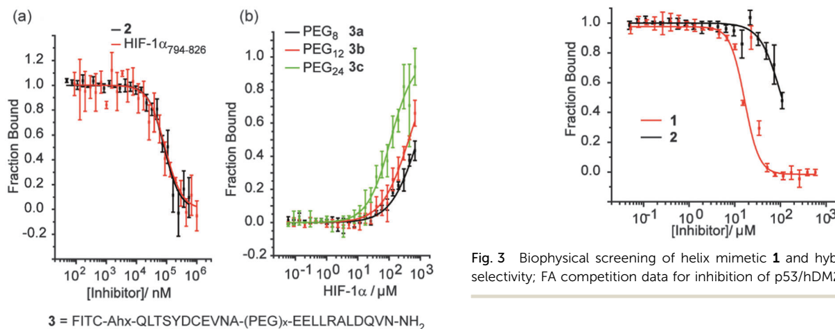
Scheme 1 (a) Structure of peptide-helix mimetic hybrid 2 and 3a–3c (PEG = polyethylene glycol), (b) synthetic route for assembly of the key N-terminal Fmoc glycy 3-butyloxy-4-aminobenzoic acid building block 8 (c) outline of approach used to synthesise hybrid 2 .
