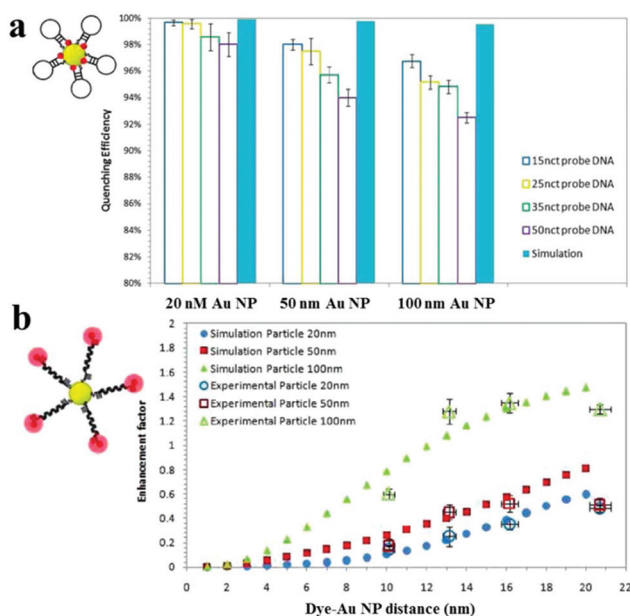
Fig. 7 Fluorescence quenching and enhancement by Au NP size and dye–Au NP distance. (a) Quenching efficiency as a function of Au NP size and DNA length. (b) Enhancement factor as a function of particle size and dye–Au NP distance. Reprinted with permission from ref. 161. Copyright 2011, American Chemical Society.
