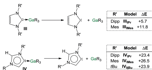
Fig. 7 Estimated dissociation energies ( \text{kcal mol}^{-1} ) of complexes III and IV ( \text{R} = \text{Dipp, Mes, I}^t\text{Bu} ).
