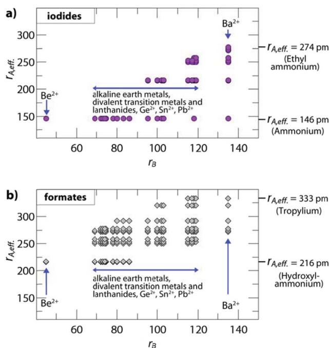
Fig. 2 Plotted are the effective radii of protonated amines r_{A,eff} vs. ionic radii of the divalent metals r_B of hypothetical compositions. The figure shows (a) iodide based and (b) formate based permutations with TFs between 0.8 and 1.0. The plots highlight the influence of the linking anion on the size-ranges of protonated amines and divalent metals where a hybrid perovskite structure is expected to form. The anisotropy of the anti-anti bridged formate and the associated smaller effective radius ( r_{X,eff} ) leads to a larger ReO_3 -like cavity, so that larger protonated amines can fit within the cavity for a fixed divalent metal. In the case of formates with a 4^{12} \cdot 6^3 topology and syn-anti connectivity, the size of the ReO_3 cavity is reduced and even smaller protonated amines lead to a perovskite-like architecture, as recently shown for [NH_4]Cd(HCOOH)_3 . 21
