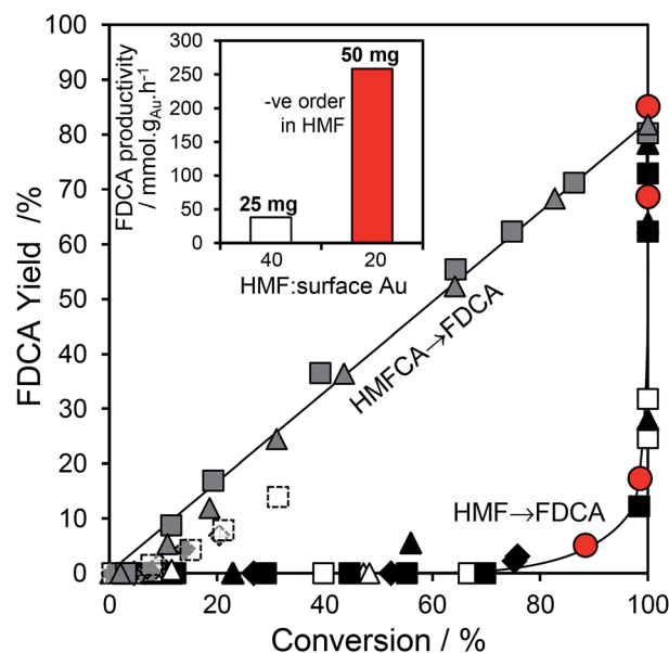
Fig. 5 (main) Disparate evolution of FDCA yield as a function of either HMF or HMFCa conversion over 25 mg ( \Delta , \nabla ) 0.5 wt%, \blacklozenge , \blacklozenge 1 wt%, \square , \square 2 wt%, \blacksquare , \blacksquare 5 wt%, and \blacktriangle , \blacktriangle 10 wt% Au/HT catalysts, and 50 mg \bullet 2 wt% Au/HT; (inset) normalised FDCA productivity per Au atom as a function of HMF : surface Au molar ratio for 2 wt% Au/HT highlighting self-poisoning by high HMF concentrations.
