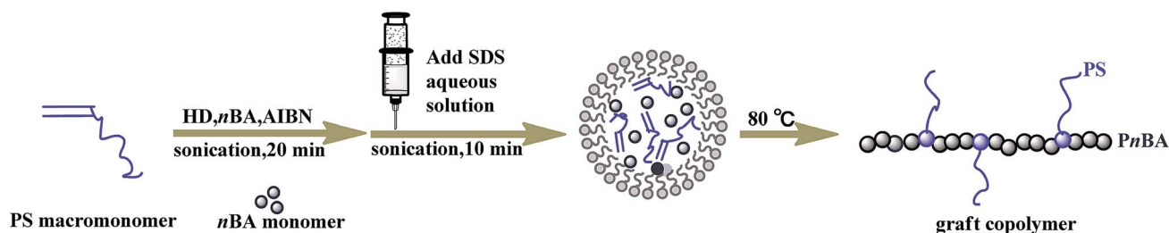
Scheme 2 Scheme for synthesis of graft copolymers poly( n -butyl acrylate)- g -polystyrene by miniemulsion polymerization using PS macromonomer.
