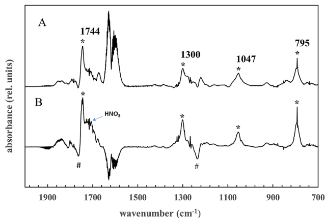
Fig. 5 Trace A shows the spectrum obtained at the end of the irradiation a \text{AA}/\text{Cl}_2/\text{NO}_x reaction mixture after subtraction of acetoxycetaldehyde, acetic acid, formic acetic anhydride and nitric acid. The * symbols in are attributed to the formation of acetoxycetyl peroxyxynitrate. Trace B is the difference spectrum obtained after subtraction of the first spectrum in which the AA was zero from the last spectrum in the experiment. This spectrum demonstrates the secondary decay of the main product acetoxycetaldehyde (# symbols) and the formation of acetoxycetyl peroxyxynitrate (* symbols).
