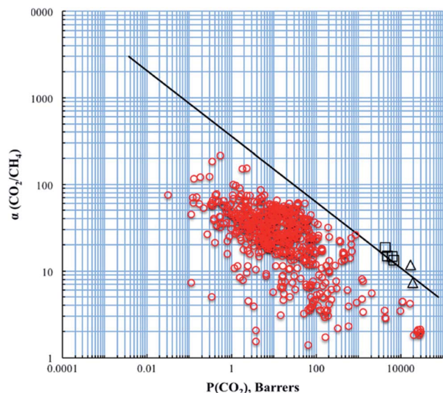
Fig. 17 Correlation of permeability and permselectivity for \text{CO}_2/\text{CH}_4 gas pair. The solid line is the Robeson upper bound of 2008. triangles indicate pim-1/zif-8 films after ethanol treatment, squares pim-1/zif-8 films as cast.
