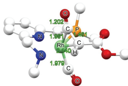
Fig. 4 DFT optimized structure of N^H1INT6 (bond lengths in Å).
