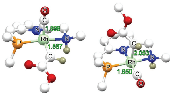
Fig. 2 DFT optimized structure of, left: N^H1INT2^b , right: N^H1INT2^a (bond lengths in Å).
