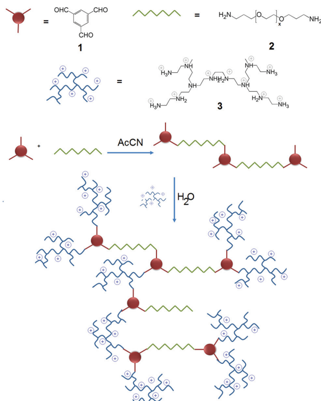
Scheme 1 Schematic representation of the synthesis of DCFs combining 1,3,5-benzenetrialddehyde cores 1 (red circle) with PEG 2 (green) in acetonitrile. Further treatment of this mixture with positively charged PEI 3 , heads (blue) in water generates DCFs. All the reactions have been performed for different molar ratios of components – see the text for details.
