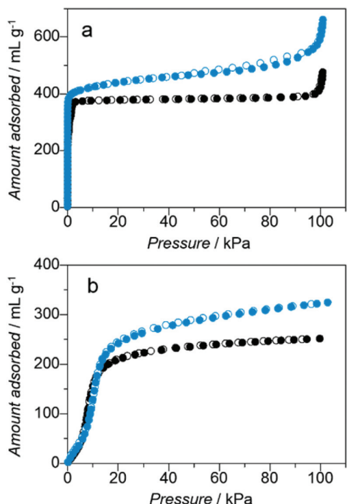
Fig. 2 Adsorption (solid circles) and desorption (open circles) of Mg-ZIF-8 (blue) and Zn-ZIF-8 (black) for (a) N_2 at 77 K and (b) CO_2 at 195 K.
