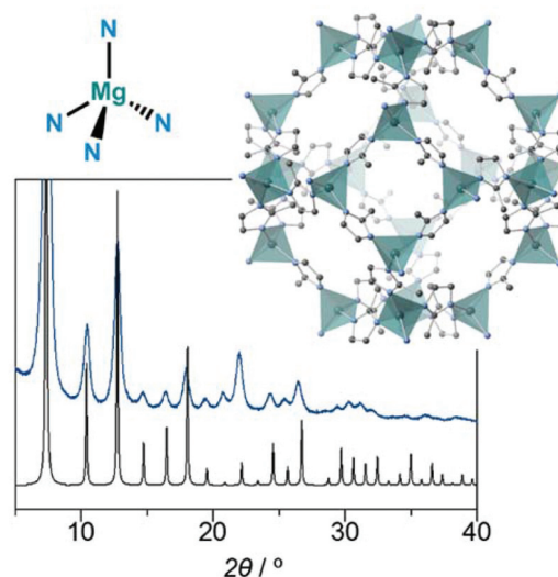
Fig. 1 Powder X-ray diffraction pattern of \text{Mg-ZIF-8} (blue) under an Ar atmosphere and the pattern of \text{Zn-ZIF-8} simulated from its single-crystal structure (black). The crystal structure of \text{Zn-ZIF-8} and the tetrahedral \text{Mg}^{2+}\text{-N} coordination geometry are also shown.
