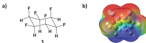
Fig. 2 (a) Structural representation of all- cis 1,2,3,4,5,6-hexafluorocyclohexane (3). (b) Electrostatic potential (ESP) of 3 [B3LYP-D3/def2-TZVP] color-coded on a scale from -0.03 au (red) to +0.03 au (blue) and mapped onto an isodensity surface \rho = 0.001 au.
