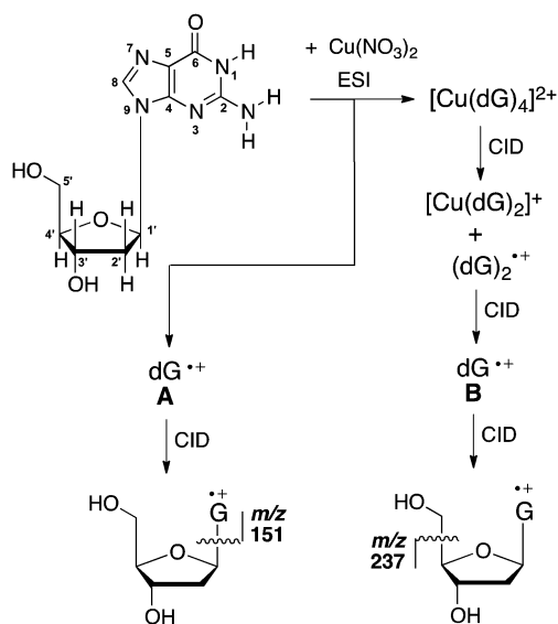
Scheme 1 Structure and atom numbering of the anti form of the neutral keto isomer of deoxyguanosine (dG), together with the experimental procedure for the formation of isomeric dG •+ species ( A and B ) via ESI/MS n , and their resultant fragmentation channels under conditions of collision-induced dissociation (CID).
