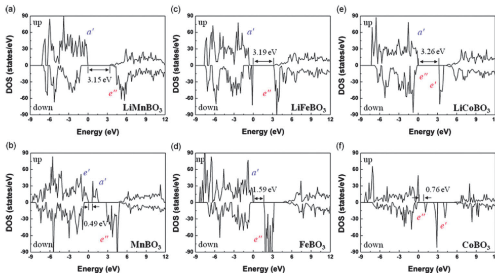
Fig. 19 DOS of \text{Li}_x\text{MBO}_3 ( x = 1, 0 ; \text{M} = \text{Mn, Fe, Co} ). Highest occupied bands, lowest unoccupied bands, and bandgaps are presented. Reprinted with permission from ref. 223. Copyright 2011 American Physical Society.
