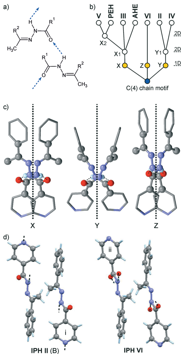
Fig. 8 a) Schematic representation of the N-H \cdots O=C-bonded C(4) chain motif (IPH: R^1 = 4-pyridyl, R^2 = phenyl) and b) tree diagram according to ref. 45 which summarises packing relationships between crystal structures; c) N-H \cdots O=C bonded chains of the geometry types X (III), Y (IV) and Z (VI), viewed along their respective translation vector (dotted lines indicate an axial glide plane with a glide vector of 1/2 of the lattice vector normal to the projection plane); d) centrosymmetric dimer units present in the IPH polymorphs II (molecule B) and VI [symmetry operations: (i) 1 - x, -y, 1 - z and (ii) 1 - x, -y, -z ].
