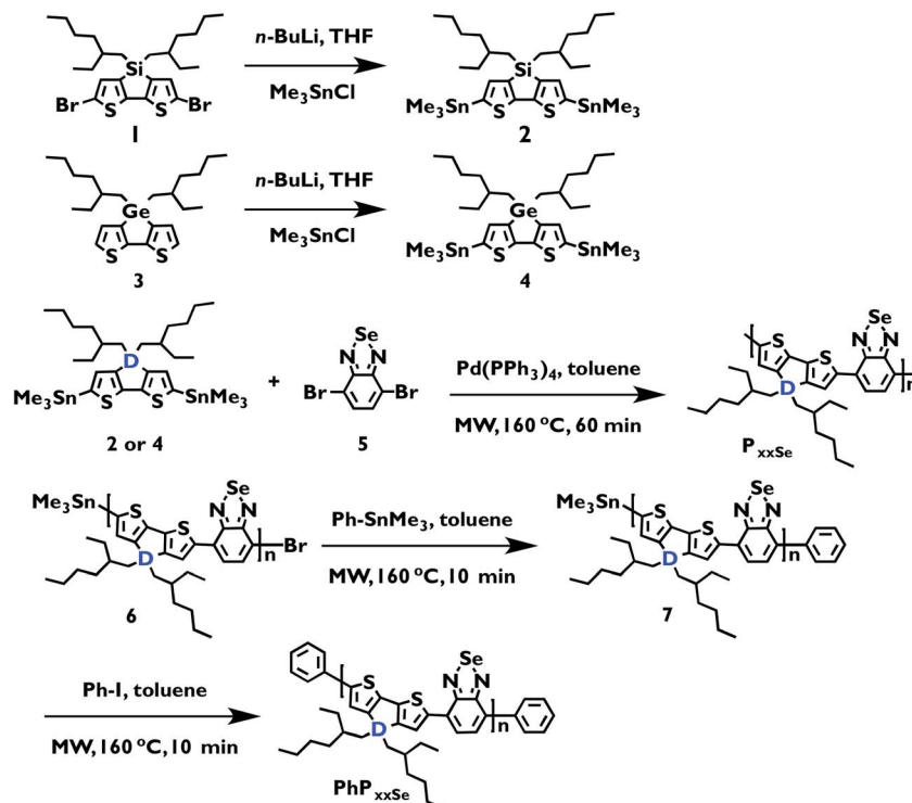
Scheme 1 Synthesis of heavy atom monomers and corresponding 2,1,3-benzoselenadiazole-containing polymers P_{SiSe} ( D = Si ), P_{GeSe} ( D = Ge ); MW = microwave.
