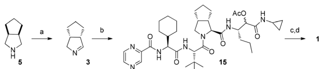
Fig. 5 Synthesis of 1. Reagents and conditions: (a) monoamine oxidase (MAO-N), 100 mM \text{KPO}_4 buffer, pH = 8.0, 37^\circ\text{C} ; (b) 2, 4, \text{CH}_2\text{Cl}_2 , 76%; (c) \text{K}_2\text{CO}_3 , MeOH; (d) DMP, \text{CH}_2\text{Cl}_2 , 80% over two steps. DMP = Dess–Martin periodinane.
