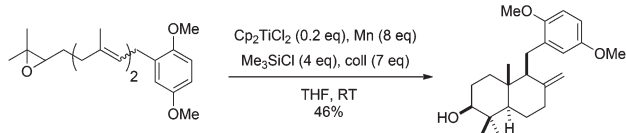
Scheme 56 Straightforward access to meroterpenes.
