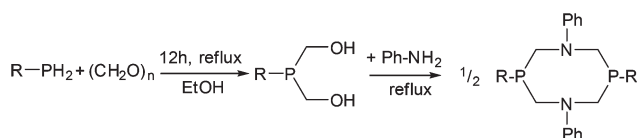
Scheme 2 Synthesis of cyclic bisphosphine ligands a–d ( P^R_2N^{Ph}_2 ) starting from primary phosphines and aniline: a : R = Ph (phenyl), b : R = Bn (benzyl), c : R = Cyc (cyclo-hexyl) and d : R = tBu (tert-butyl).
