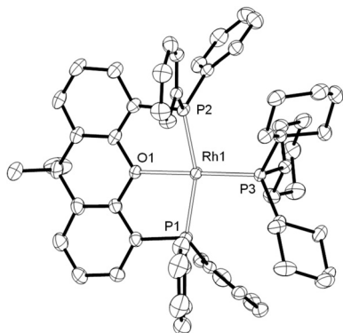
Fig. 4 Solid state structure of the cationic portion of 8 . [\text{BAR}^{\text{F}}_4]^- anion and H atoms are omitted for clarity. Displacement ellipsoids are drawn at the 50% probability level. Selected bond lengths (Å) and angles (°): Rh1–P1, 2.2854(7); Rh1–P2, 2.2923(7); P3–Rh1, 2.2611(7); Rh1–O1, 2.2395(19); P2–Rh1–P1, 159.70(3); P3–Rh1–O1, 170.44(6).
