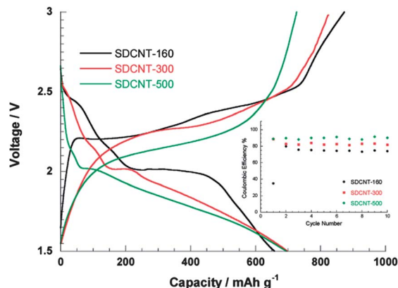
Fig. 8 Discharge-charge profiles of the second cycles and (inset) Coulombic efficiency under 10 \text{ mA g}^{-1} for DCNT-S composites synthesized at 160, 300 and 500^\circ\text{C} . 47 Reproduced from ref. 47. Copyright 2011 American Chemical Society.
