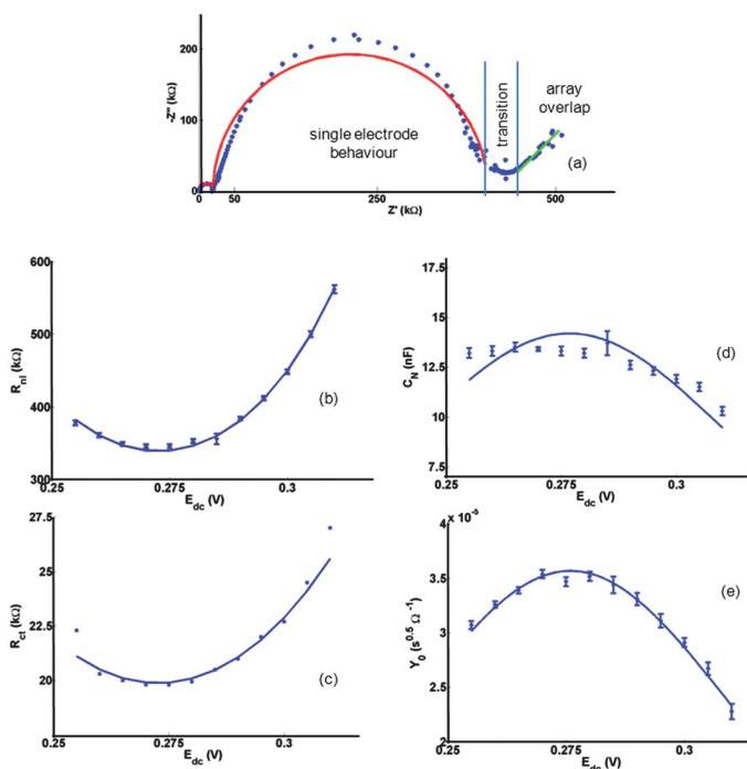
Fig. 7 (a) Typical subtracted Nyquist Electrochemical Impedance Spectroscopy (EIS) data at the 10\mu 3D50n electrode for oxidation of FCA(I) solution at E_{dc} = +0.290 V. Also shown are theoretical fits to the circuit in Fig. 4c and to the circuit (resistance in series with Warburg element) appropriate at low frequency when there is complete diffusional array overlap. Fits (solid lines) to the (b) R_{nl} (c) R_{ct} (d) C_N (e) Y_0 data extracted from iterative fitting to the EIS measurements at each E_{dc} performed using either Matlab (The Mathworks, Natick, Massachusetts, USA) or Nova (Version 1.9, Metrohm Autolab B.V., Utrecht, The Netherlands). The fits of these data to eqn (3), (8), (10) and (13), (lines shown in (b), (c), (d) and (e)) gave the following global values: E' = 0.273 \pm 0.002 V; R_{ct}^{min} = 19.87 \pm 0.06 k \Omega ; R_{nl}^{min} = 339 \pm 1 k \Omega ; C_N^{max} = 14.3 \pm 0.3 nF; Y_0^{max} = 35.7 \pm 0.2 \mu s^{0.5} \Omega^{-1} .
