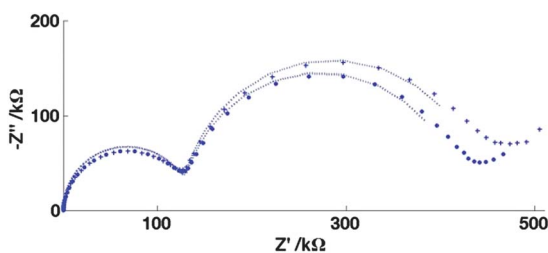
Fig. 11 EIS data for the 20\mu\text{m} electrode showing the oxidation of 0.1 mM FCA in FCA(I) solution (+) and FCA(II/10) solution (●) and the corresponding fits for E_{dc} = E' , V_{ac} = 10 \text{ mV} , for the frequency range 100 kHz to 10 mHz (logarithmic distribution). Fits: FCA(I) solution: R_{ct} = 135 \pm 1 \text{ k}\Omega , C_{dl} = 31.1 \pm 0.7 \text{ nF} , R_{nl}^{\text{min}} = 309 \pm 3 \text{ k}\Omega , C_N = 1.34 \pm 0.02 \mu\text{F} , FCA(II/10) solution: R_{ct} = 135 \pm 1 \text{ k}\Omega , C_{dl} = 27.7 \pm 0.6 \text{ nF} , R_{nl}^{\text{min}} = 283 \pm 2 \text{ k}\Omega , C_N = 1.33 \pm 0.02 \mu\text{F} .
