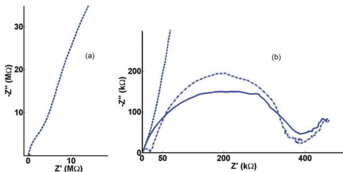
Fig. 6 (a) Nyquist Electrochemical Impedance Spectroscopy (EIS) data for oxidation of FCA in FCA(I) solution at the 10\mu 3D50n electrode at E_{dc} = +0.275 V, frequencies logarithmically spaced between 100 kHz and 0.01 Hz and an ac perturbation of 10 mV. (b) Same data on an expanded scale for background electrolyte (dashed line), redox solution (solid line) and the subtracted impedance (dash dotted line).
