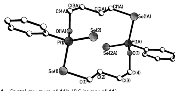
Fig. 4 Crystal structure of 11b ( R,S isomer of 11 ).
