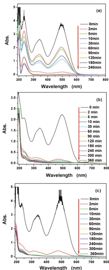
Fig. 5 UV-Vis absorption spectra of CR solutions (CRS) before and after treatment with \text{CeO}_2 at different time intervals: (a) CRS ( 100 \text{ mg L}^{-1} , 50 mL) in the presence of 250 mg of \text{CeO}_2 nanoparticles, (b) CRS ( 50 \text{ mg L}^{-1} , 50 mL) in the presence of 20 mg of \text{CeO}_2 nanorods, and (c) CRS ( 80 \text{ mg L}^{-1} , 50 mL) in the presence of 150 mg of the \text{CeO}_2 mixture of nanoparticles and nanorods.
