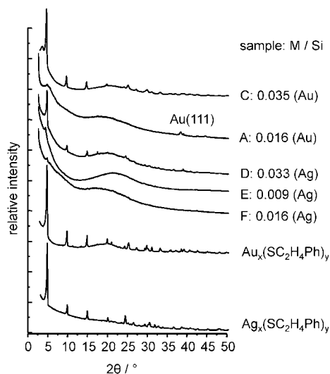
Fig. 1 XRD patterns of gold and silver particles stabilized by phenylthiol and with different loadings.
