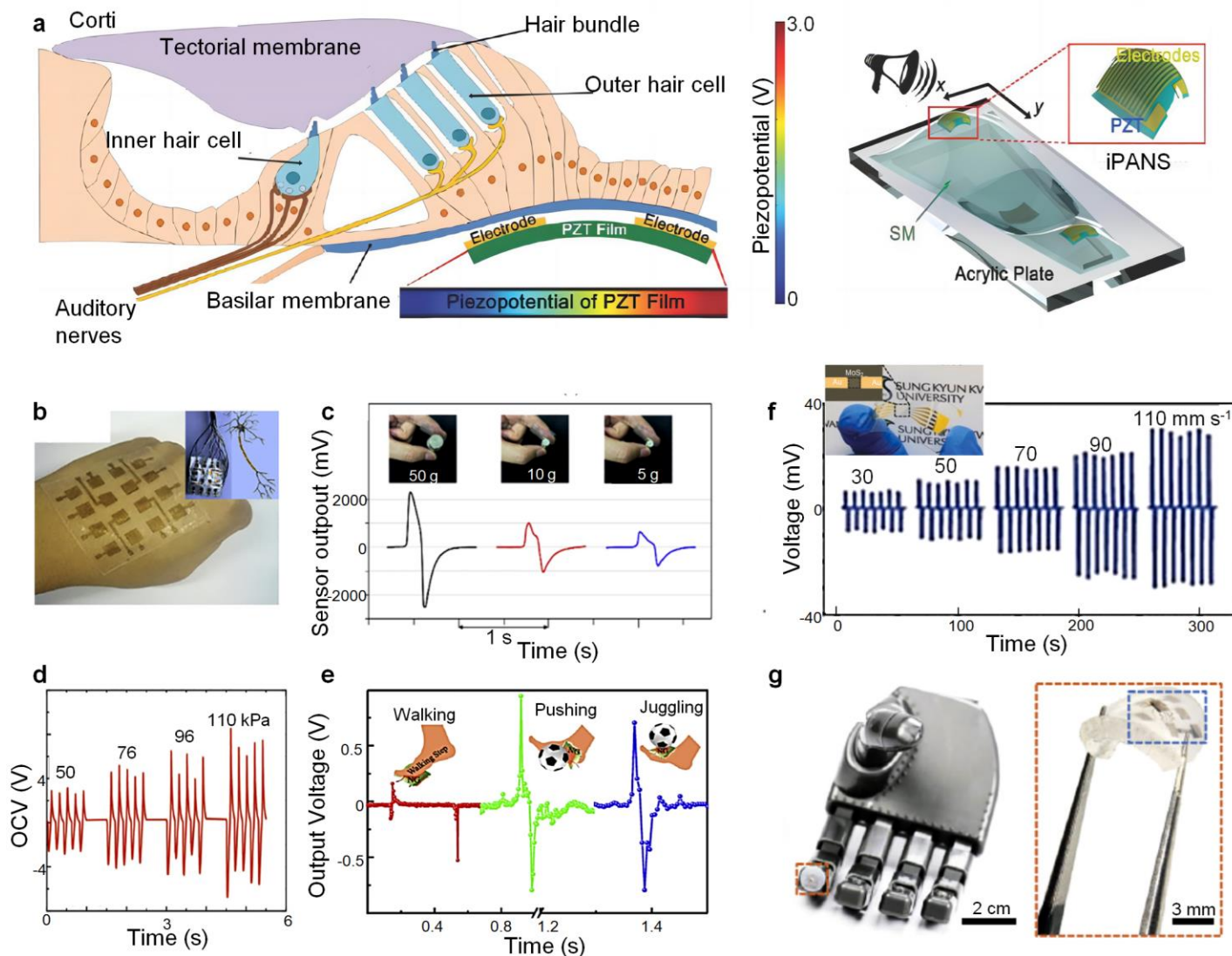
Fig. 5. AI-integrated PENGs for wearables and robotics. (a) Biomimetic inorganic piezoelectric acoustic nanosensor. 216 Copyright 2014, Wiley. (b,c) Multi-sensing e-skin for pressure and temperature detection. 236 Copyright 2018, ACS. (d) Output voltage and pressure for affordable e-skin. 112 Copyright 2020, IOPscience. (e) Wearables inspired by the fish swim bladder. 237 Copyright 2018, Wiley. (f) MoS 2-x -based PENG under different bending speeds. 241 Copyright 2018, Wiley. (g) Implanted microsystem in a robotic hand. 213 Copyright 2019, Springer Nature.
