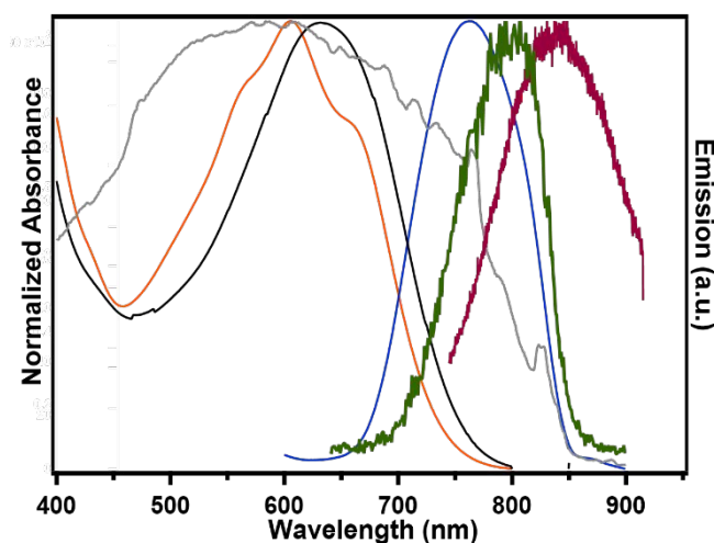
Figure 2. Vis-NIR absorption/fluorescence of LDBC encapsulated II-EDOT-TPA (orange and blue traces) and solid-state II-EDOT-TPA (grey and purple traces) and II-EDOT-TPA in 6 \times 10^{-5} M \text{CHCl}_3 (black and green traces)
