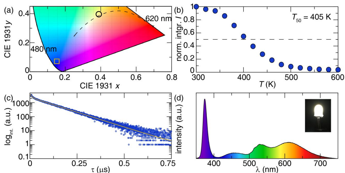
Figure 5. (a) CIE diagram for \text{Cs}_2\text{NaInCl}_6:\text{Sb}^{3+} , where the CIE coordinates (0.148, 0.067) are marked with a square. (b) Normalized, integrated intensity of the emission as a function of temperature. (c) Lifetime measurements of sample (6). (d) The luminescence spectrum of a prototype pc-LED composed of a near UV-LED ( \lambda_{\text{ex}} = 370 \text{ nm} ), and three phosphors: \text{Cs}_2\text{NaInCl}_6:\text{Sb}^{3+} , \text{Sr}_2\text{Si}_5\text{N}_8:\text{Eu}^{2+} and \beta\text{-SiAlON}:\text{Eu}^{2+} . The inset is the photograph of the white pc-LED under a forward bias of 20 mA. The circle on the CIE diagram in part (a) shows the CIE coordinates (0.3890, 0.4009) of this pc-LED.
