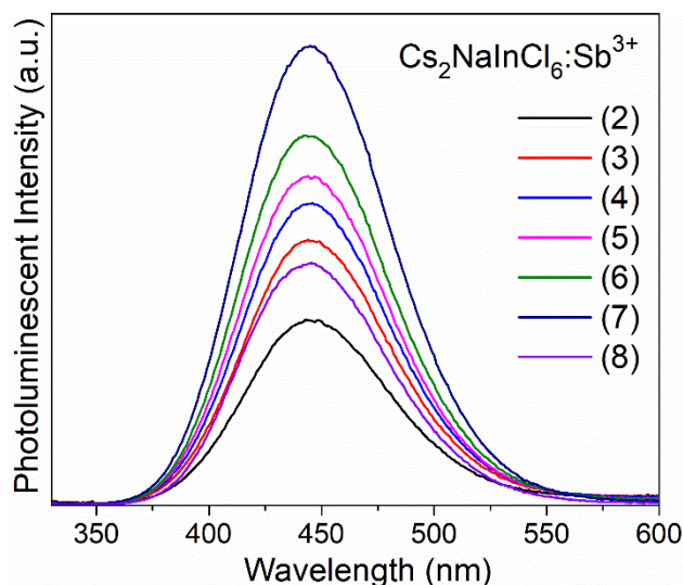
Figure 4. Emission spectra of \text{Cs}_2\text{NaInCl}_6:\text{Sb}^{3+} samples.
