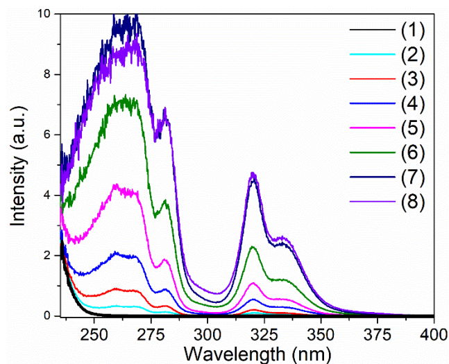
Figure 2. Pseudo-absorbance obtained from Kubelka-Munk transformation of the diffuse reflectance data of \text{Cs}_2\text{NaInCl}_6:\text{Sb}^{3+} for samples with various concentrations of \text{Sb}^{3+} .
