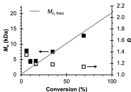
Figure 5. Evolution of molecular weight (filled squares) and \bar{D} (hollow squares) for eO-ATRP using a vycor-glass frit to separate the counter electrode from the polymerization solution. Conditions: [MMA]:[DBMM]:[1] = [1000]:[5]:[0.1], 2 mL MMA, 2 mL DMAc, SE = 0.1 M LiPF 6 . Reaction performed in a 5-neck pear flask and irradiated with an 80 mm x 40 mm white LED well (9 LED segments, see Experimental Equipment in SI). Working electrode = glassy carbon, counter electrode = Pt wire, reference electrode = Ag/AgNO 3 , and E_{app} = E_{1/2} - 120 mV.
