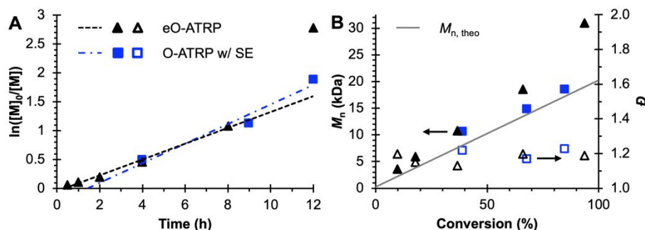
Figure 3. Plot of the natural logarithm of monomer (M) consumption over time (A). Molecular weight (filled markers) and \bar{D} (hollow markers) evolution (B) for eO-ATRP (black triangles) and O-ATRP with supporting electrolyte (blue squares). Conditions: [MMA]:[DBMM]:[1] = [1000]:[5]:[0.1], 2 mL MMA, 2 mL DMAc, SE = 0.094 M Bu _4 NPF _6 and 0.006 M Bu _4 NBr. Reactions performed in a U-cell and irradiated with a high-power white LED (see Experimental Equipment in SI). For eO-ATRP, working electrode = glassy carbon, counter electrode = Pt wire, reference electrode = Ag wire quasi-reference electrode, and E_{\text{app}} = E_{1/2} - 120 mV.
