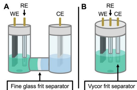
Figure 4. Diagram of the apparatus used in this work. Originally, a modified U-cell was employed to separate the working and counter electrode compartments (A). When this separator was found to be ineffective on the time scale of eO-ATRP, a new apparatus was developed using a 5-neck electrochemical flask (see Experimental Equipment in SI) and vycor frit separators to isolate the counter electrode (B). WE = working electrode, RE = reference electrode, and CE = counter electrode.
