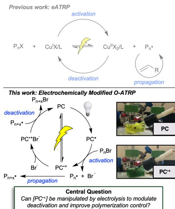
Figure 1. Previous work demonstrated the ability to mediate ATRP using electrochemistry (top). In this work (bottom), we ask whether this principle can be applied to O-ATRP to control the concentration of PC^{•+} and thereby control deactivation in this polymerization method. Figure inset (bottom right) demonstrates the conversion of PC to PC^{•+} using potentiostatic bulk electrolysis.
