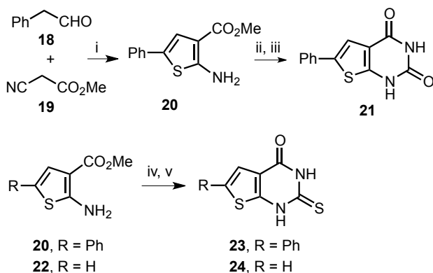
Scheme 3 Synthesis of thieno[2,3- d ]pyrimidine-2,4(1 H ,3 H )-dione and 2-thio-2,3-dihydrothieno[2,3- d ]pyrimidin-4(1 H )-one analogs. Reagents and conditions: (i) S_8 , Et_3N , DMF, room temperature, 21 h, 90%; (ii) ClSO_2NCO , CH_2Cl_2 , -78^\circ C to room temperature, 40 min; (iii) [a] dioxane/ H_2O , room temperature to 85^\circ C , 45 min; [b] aqueous NaOH, 85^\circ C , 30 min; [c] aqueous HCl, room temperature, 57% (2 steps); (iv) BzCl , NH_4NCS , CH_3CN , reflux, 6 h, 69% (R = Ph), 67% (R = H); (v) [a] KOH, EtOH, reflux, 14–19 h; [b] aqueous HCl, room temperature, 49% ( 23 ), 57% ( 24 ).
