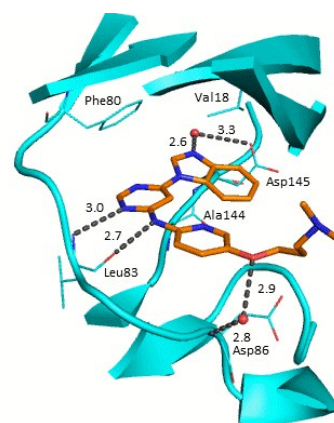
Fig. 2 X-ray co-crystal structure of 4 bound to CDK2. Measurements in Å. PDB ID 4BZD.
