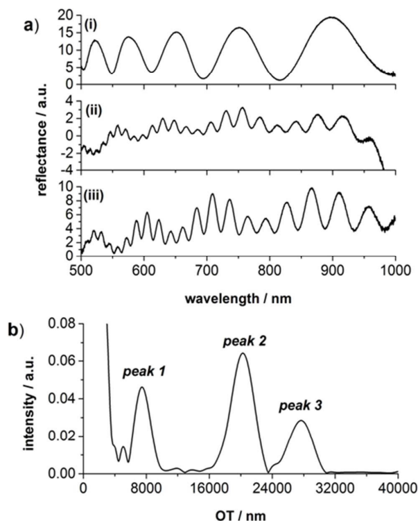
Figure 3. Optical characterization of the fabricated PSi structures. a) After each production step a reflectance spectrum was recorded. Here, i) is the spectrum of the structure obtained by etching with EES, ii) spectrum of the structure after the second etch step with WES, iii) spectrum of the PSi structure after gold removal. b) The inverse spectrum of the reflectance spectrum of the PSi structure was analyzed using fast Fourier transform in order to obtain the characteristic OT peaks.
