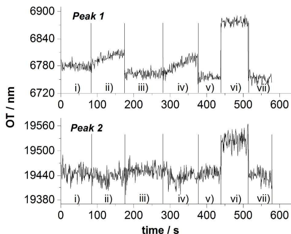
Figure 4. Optical response of the presented PSi sensor expressed as changes in the OT. Peak 1 corresponds to the OT of the pillar top layer and peak 2 is related to the OT of PSi bottom layer with smaller pores. The following solutions were consecutively flown over the sensor surface: i) PBS pH 7.4, ii) 0.25 mg/mL protein A in PBS, iii) PBS pH 7.4, iv) 0.25 mg/mL protein A in PBS, v) PBS pH 7.4, vi) 20% w:w sucrose in PBS, vii) PBS pH 7.4.
