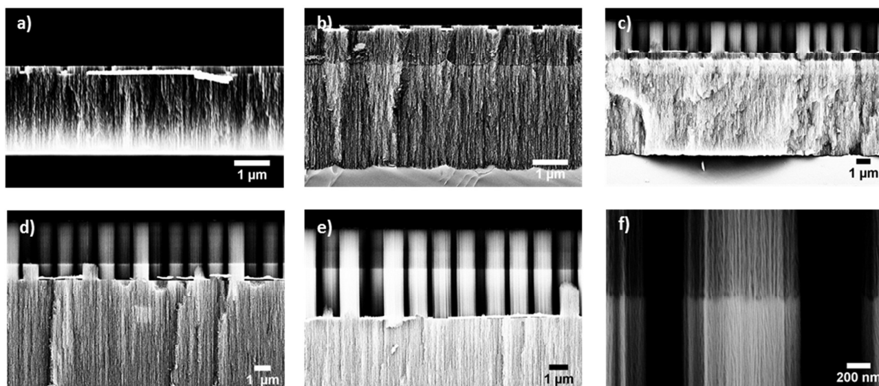
Figure 2. Cross sectional SEM images of the fabricated PSi structures. (a) PSi monolayer: EES, etched for 75s); (b) PSi bilayer: EES 75s, WES 90s; (c) PSi-pillars bilayer: EES 75s, WES 120s; (d) PSi-pillar bilayer: EES 75s, WES 150s; (e) PSi-pillar bilayer: EES 75s, WES 160s; (f) magnification of the pillar interface.
