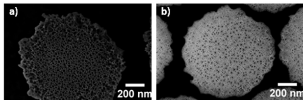
Figure 1. Top view SEM images of PSi pillars obtained from gold-patterned Si substrates after MACE treatment with two different etching solutions: (a) ethanol/HF/H 2 O 2 and (b) water/HF/H 2 O 2 .
