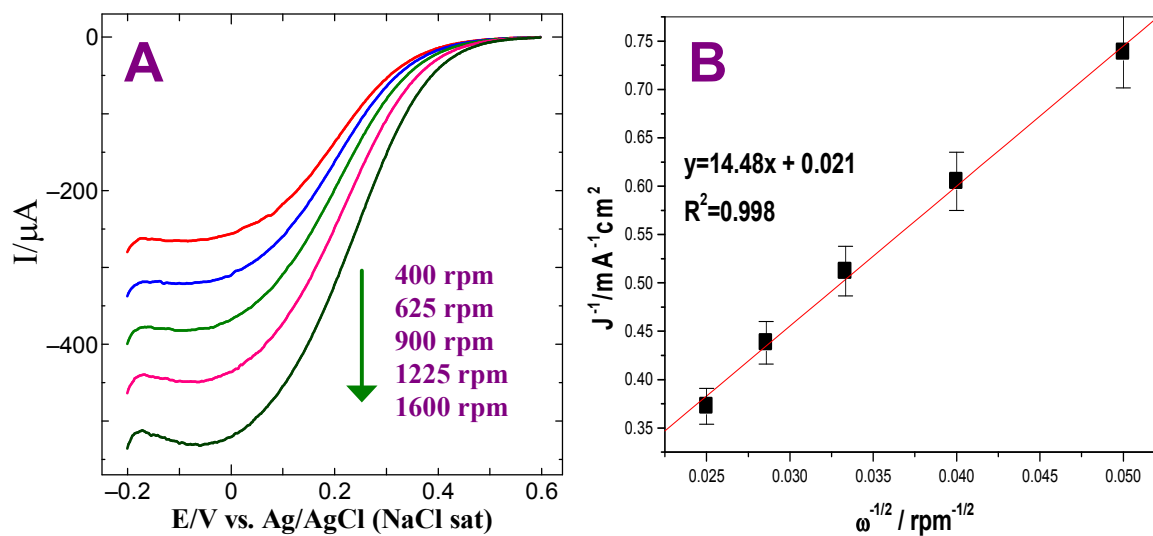
Figure 5. (A) Steady-state voltammograms for the ORR obtained at GC/Au@PtNPs electrode in \text{O}_2 saturated 0.5 M \text{H}_2\text{SO}_4 . Rotation rate: 400, 625, 900, 1225 and 1600 rpm. Scan rate: 50 \text{ mV s}^{-1} . (B) Corresponding K-L plot.
