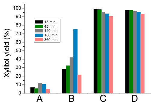
Figure 3. Xylitol yield during different reaction times at 120°C.
