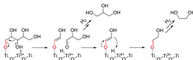
Figure 7. \text{Ti}^{3+} acting as a Lewis base for xylose retro-aldol reaction to glycols.
