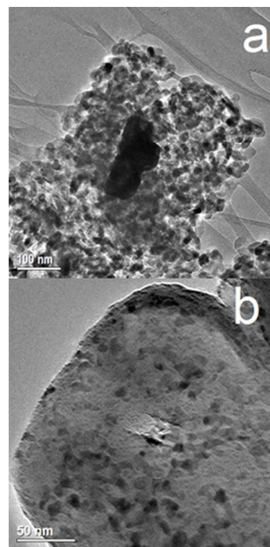
Figure 5. The TEM images of catalysts A (a) and C (b) show the agglomeration of the Ru on the anatase support.
