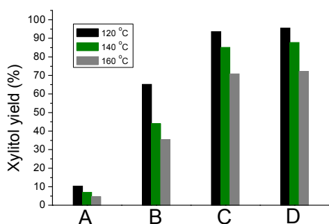
Figure 1. Xylitol yield at different temperatures after 3 h reaction. Reaction conditions: 20 bar H 2 , xylose:Ru ratio 100:1(w/w), solvent water.
