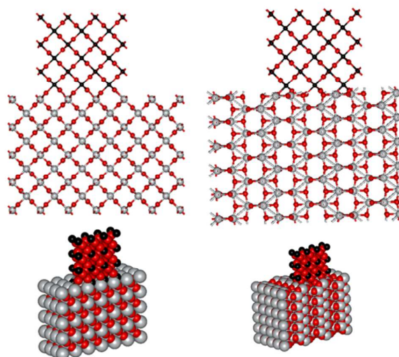
Figure 6. Atomic structures of \text{RuO}_2 on rutile (left) and anatase (right) \text{TiO}_2 showing the high degree of lattice matching of \text{RuO}_2 on rutile \text{TiO}_2 (created by viewerlite software). 50
