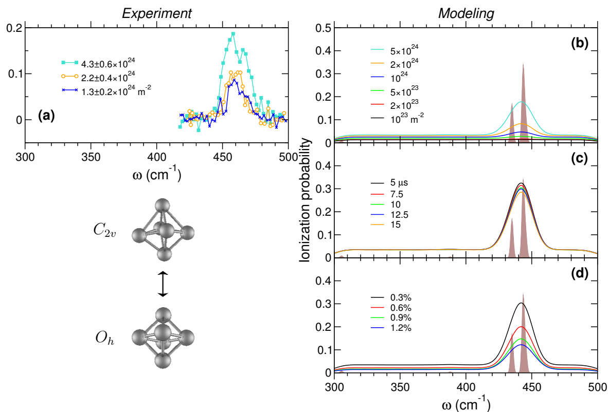
Fig. 2 Ionization probability of \text{Si}_6 as a function of laser wavelength, measured experimentally (left panel) and obtained from modeling (right panels) for different IR laser conditions. In (a) and (b) the photon exposure is varied for a macropulse duration of 8 \mu\text{s} ( 10 \mu\text{s} in the modeling) and an excitation laser bandwidth of 0.3\% ; In (c) the macropulse duration is varied at fixed photon exposure of 5 \times 10^{24} \text{ m}^{-2} ; In (d) the IR laser bandwidth is varied while the photon exposure is constant at 5 \times 10^{24} \text{ m}^{-2} and for a macropulse duration of 10 \mu\text{s} . The theoretical linear absorption spectrum at equilibrium ( 110 \text{ K} ) is superimposed on the calculated action spectra as brown histograms.
