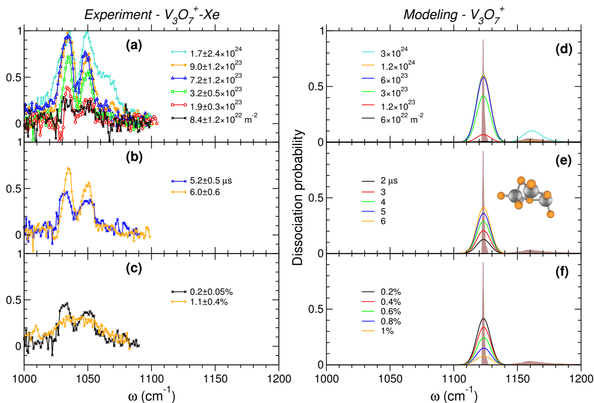
Fig. 6 Dissociation probability of the xenon atom from V_3O_7^+ + Xe as a function of laser wavelength, measured experimentally (left panel) and obtained from modeling (right panels) for different conditions of excitation. In (a) and (d) the photon exposure is varied for a macropulse duration of 6 \mu s ; In (b) and (e) the macropulse duration is varied at fixed photon exposures of 3.2 \times 10^{23} m^{-2} (experiment) and 3 \times 10^{23} (modeling); In (c) and (f) the IR laser bandwidth is varied while the photon exposures are constant with the same values as in panels (b) and (e), respectively, the macropulse duration being fixed at 5.2 \mu s (experiment) or 6 \mu s (modeling). The theoretical linear absorption spectrum at equilibrium is superimposed on the calculated action spectra as brown histograms.
