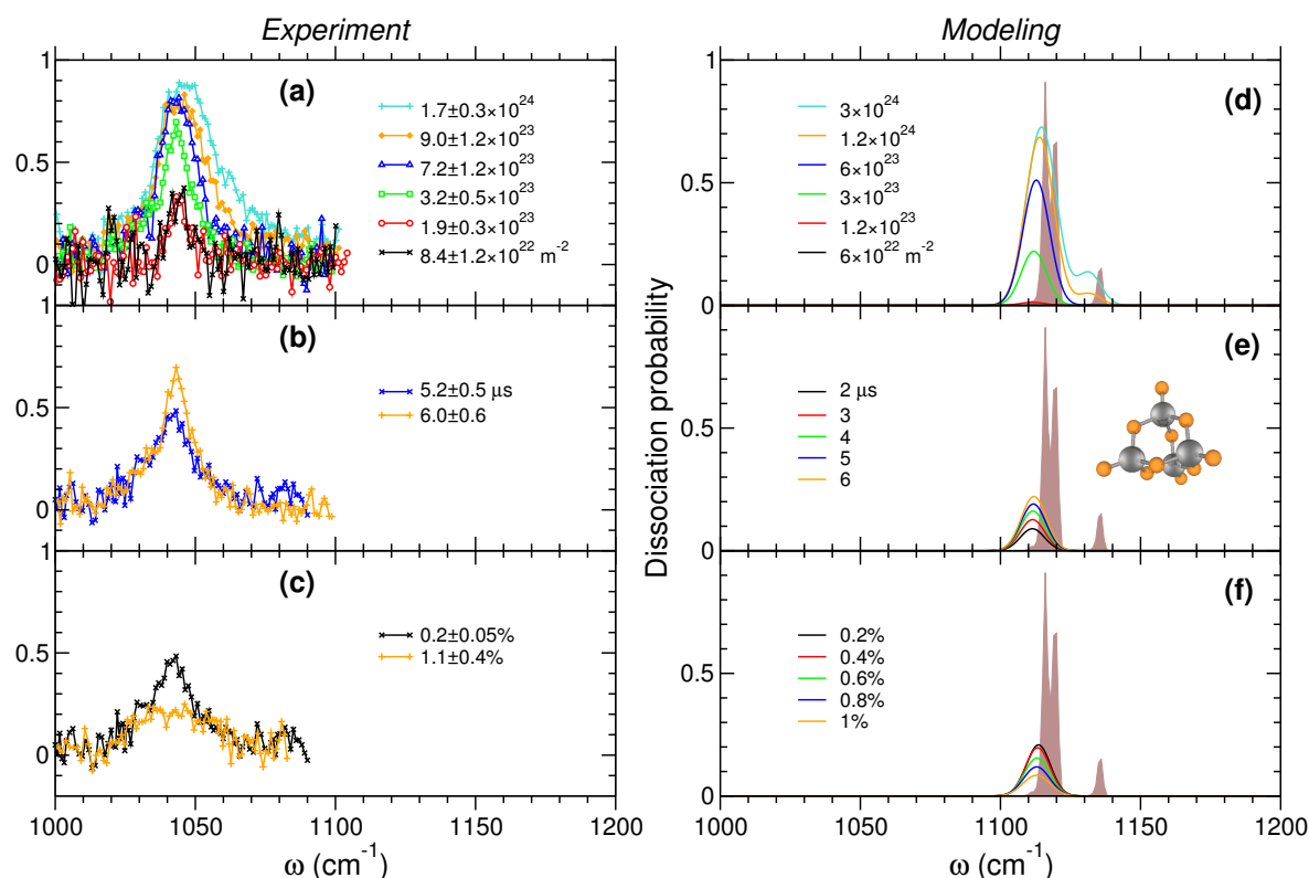
Fig. 5 Dissociation probability of V_4O_{10}^+ as a function of laser wavelength, measured experimentally (left panel) and obtained from modeling (right panels) for different conditions of excitation. In (a) and (d) the photon exposure is varied for a macropulse duration of 6 \mu\text{s} ; In (b) and (e) the macropulse duration is varied at fixed photon exposures of 3.2 \times 10^{23} \text{ m}^{-2} (experiment) and 3 \times 10^{23} \text{ m}^{-2} (modeling); In (c) and (f) the IR laser bandwidth is varied while the photon exposures are constant with the same values as in panels (b) and (e), respectively, the macropulse duration being fixed at 5.2 \mu\text{s} (experiment) or 6 \mu\text{s} (modeling). The theoretical linear absorption spectrum at equilibrium is superimposed on the calculated action spectra as brown histograms.
