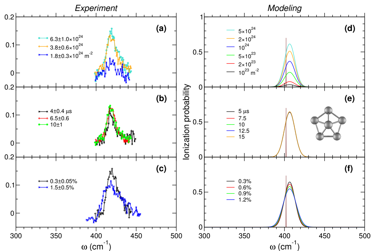
Fig. 3 Ionization probability of \text{Si}_7 as a function of laser wavelength, measured experimentally (left panel) and obtained from modeling (right panels) for different IR laser conditions. In (a) and (d) the photon exposure is varied for a macropulse duration of 10 \mu\text{s} ; In (b) and (e) the macropulse duration is varied at fixed photon exposures of 3.8 \times 10^{24} \text{ m}^{-2} (experiment) or 5 \times 10^{24} \text{ m}^{-2} (modeling); In (c) and (f) the IR laser bandwidth is varied while the photon exposures are constant at 6.3 \times 10^{24} \text{ m}^{-2} (experiment) or 5 \times 10^{24} \text{ m}^{-2} (modeling) and for a macropulse duration of 10 \mu\text{s} . The theoretical linear absorption spectrum at equilibrium is superimposed on the calculated action spectra as brown histograms.
