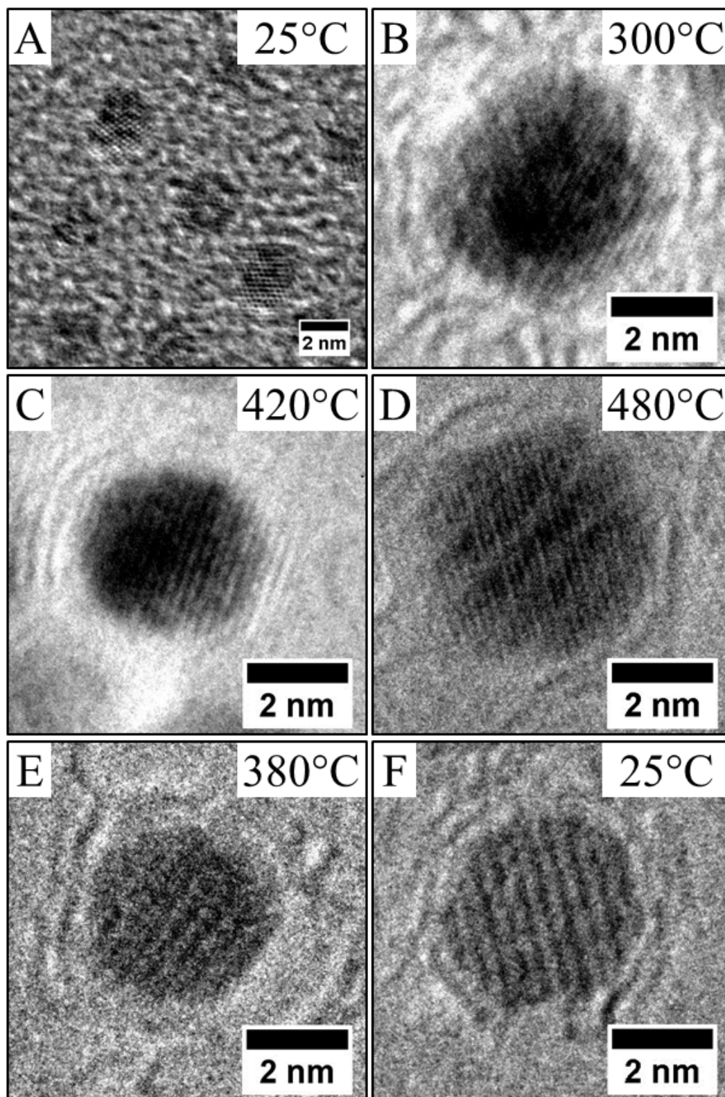
Figure 8: HRTEM images of (Co_{50}Pt_{50})_{Polyol} during annealing treatment: (A) room temperature (RT), (B) 300°C, (C) 420°C on the increasing part of the annealing and (D) 480°C, (E) 380°C and (F) RT on the decreasing part of the annealing.
