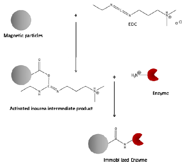
Figure 1: reaction scheme of enzyme immobilization using the zero-length crosslinking agent EDC
