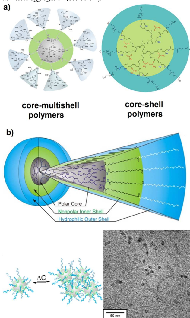
Figure 3. a) Different modification of hyperbranched polyglycerol as nanocarrier systems for drugs/dye delivery applications. b) Structure of core-multishell (PG-C18-PEG350) based on SANS data and cryo TEM. Modified from refs. 35, 37, 39-42, 44 with permission from The American Chemical Society, Elsevier B. V. and The Royal Society of Chemistry.
