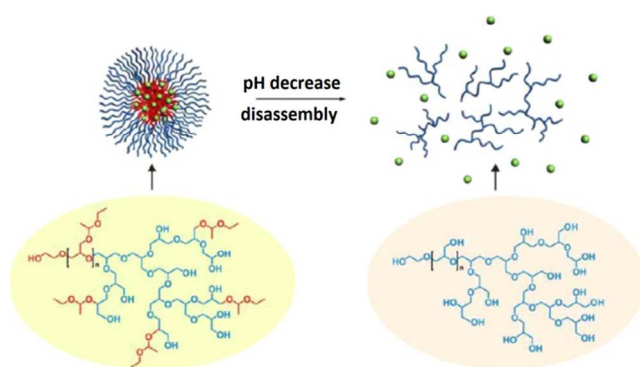
Figure 7. The disassembly of the pyrene-loaded polymeric micelle under acidic conditions. Reprinted with permission from ref. 53; Copyright 2013 American Chemical Society.
