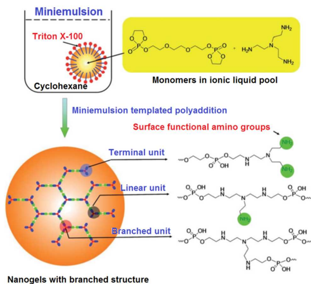
Figure 21. The synthesis of nanogels based on polyphosphates. Reproduced with permission from ref. 107; Copyright 2012 The Royal Society of Chemistry.
