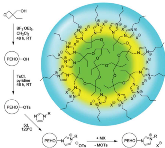
Figure 9. Routes to nanostructured hyperILs with onion-like topology and facile polarity design. Ts=p-toluenesulfonyl (tosyl). Reprinted from ref. 64, Copyright 2013, with permission from WILEY-VCH
