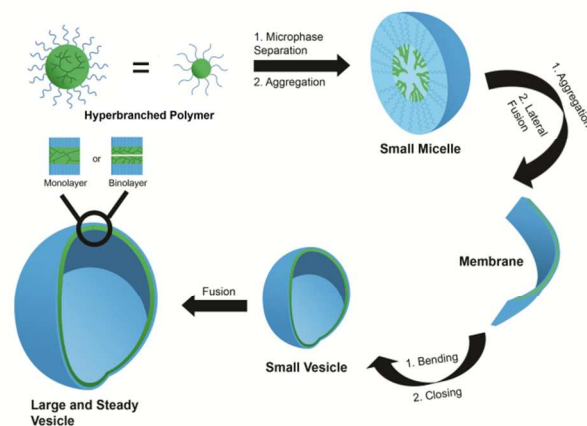
Figure 1. Schematic representation of amphiphilic hyperbranched polymers forming micelles, membrane, and vesicle. Modified from ref. 15. With permission of WILEY.
