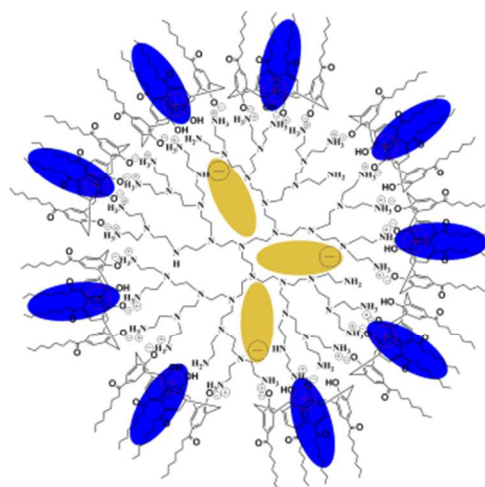
Figure 17. Structure of supramolecular hPEI-AC4 nanocarriers with encapsulated guests in isolated sites. Blue ellipses indicate methyl blue and dark yellow ellipses indicate methyl orange. Reprinted with permission from ref. 83; Copyright 2009 WILEY-VCH.
