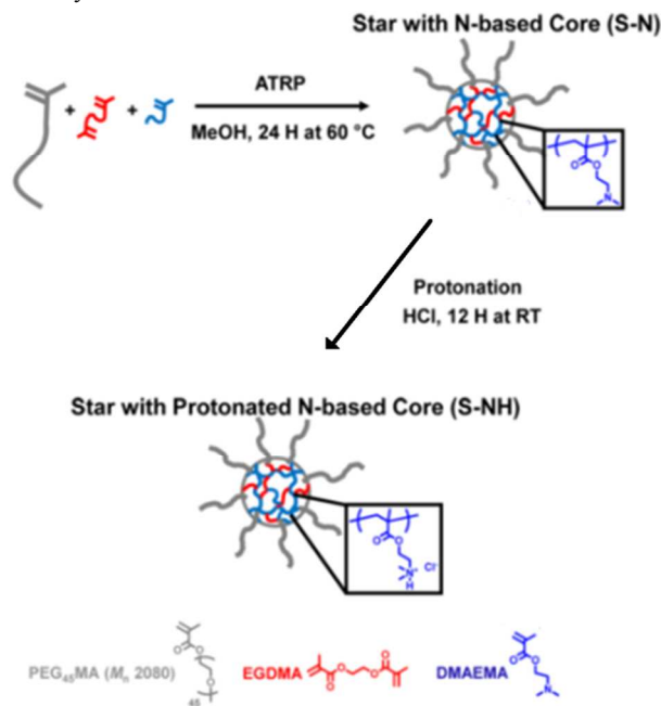
Figure 24. Synthesis of star polymers with a cationic core (S-NH) for siRNA or pDNA delivery by ATRP. Reproduced with permission from ref. 110; Copyright 2013 American Chemical Society.
