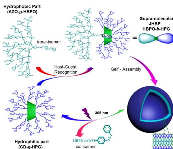
Figure 25. Self-Assembly and Disassembly Processes of the Supramolecular Janus Hyperbranched Polymer of HBPO-b-HPG. Reprinted with permission from ref. 112; Copyright 2013 American Chemical Society
