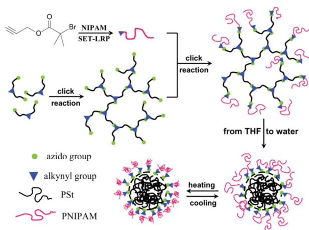
Figure 13. Synthesis strategy for star-like amphiphilic copolymers with hPS core and PNIPAm grafting chains. Reprinted with permission from ref. 75; Copyright 2013 Wiley Periodicals, Inc.
