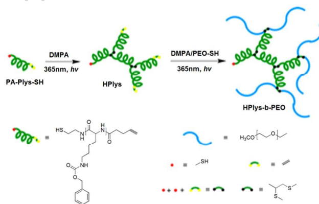
Figure 22. Hyperbranched poly( \epsilon -benzyloxycarbonyl-L-lysine) (hPlys) and the related hPlys-b-PEO block copolymer. Reproduced with permission from ref. 108; Copyright 2013 American Chemical Society.
