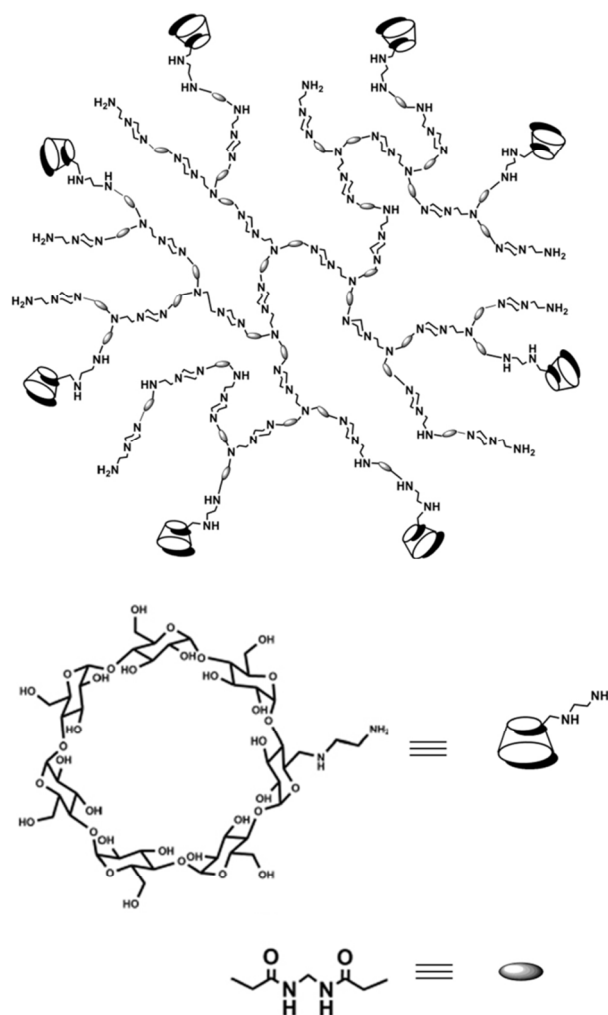
60 Figure 18. Structure of hPAA-CD polymers. Reproduced from ref. 87; Copyright 2011, with permission from the American Chemical Society.
