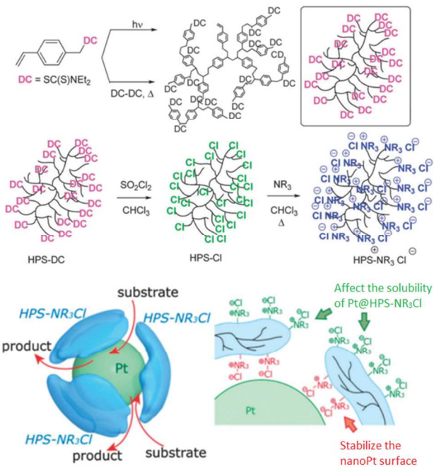
Figure 14. Hyperbranched polystyrene and the stabilization of a platinum nanoparticle by hPS-N(C 12 H 25 ) 3 + Cl - . Reproduced from ref. 76 with permission from The Royal Society of Chemistry.
