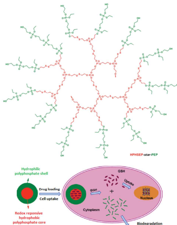
Figure 20. Structure of the amphiphilic hyperbranched copolyphosphates (upper part). Representation of the redox-responsive behavior of HPHSEP-star-PEP x micelles for intracellular drug
