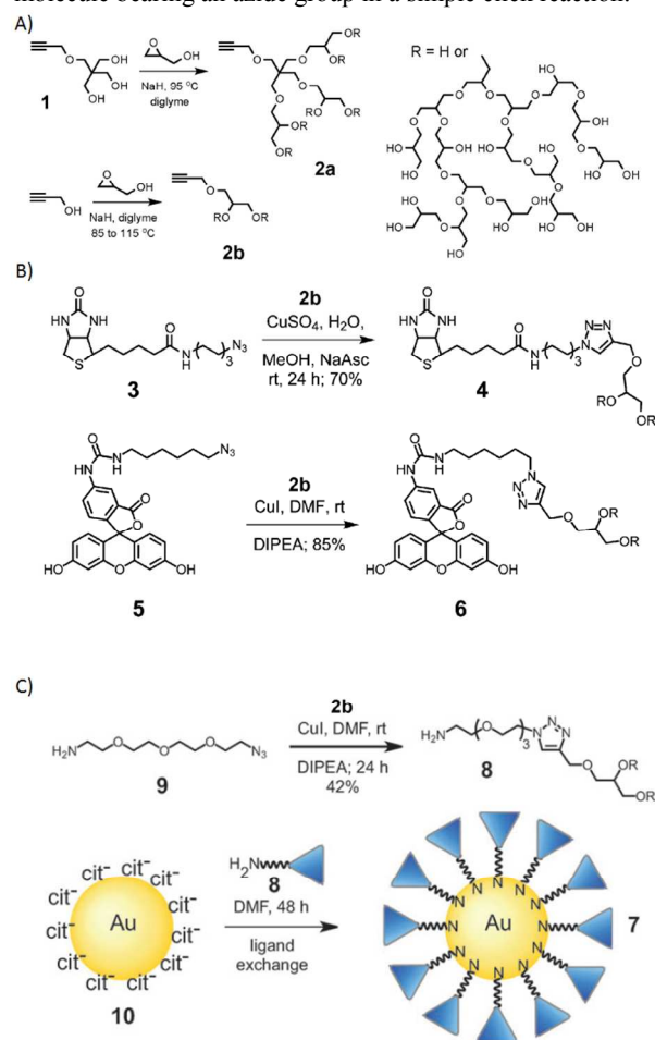
Figure 5. Clickable nanocarrier system based on hPGs. a) hyperbranched polymerization to form hPG, b) click chemistry of hPG and c) synthesis of hPG coated gold nanoparticles. Modified from ref. 50 with permission from The Royal Society of Chemistry.
