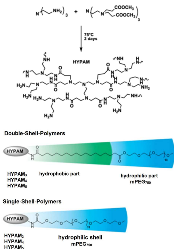
Figure 19. Structure of hyperbranched poly(amido amine) (HYPAM) polymers. Adapted from ref. 94 with permission from the American Chemical Society and The Royal Society of Chemistry.
