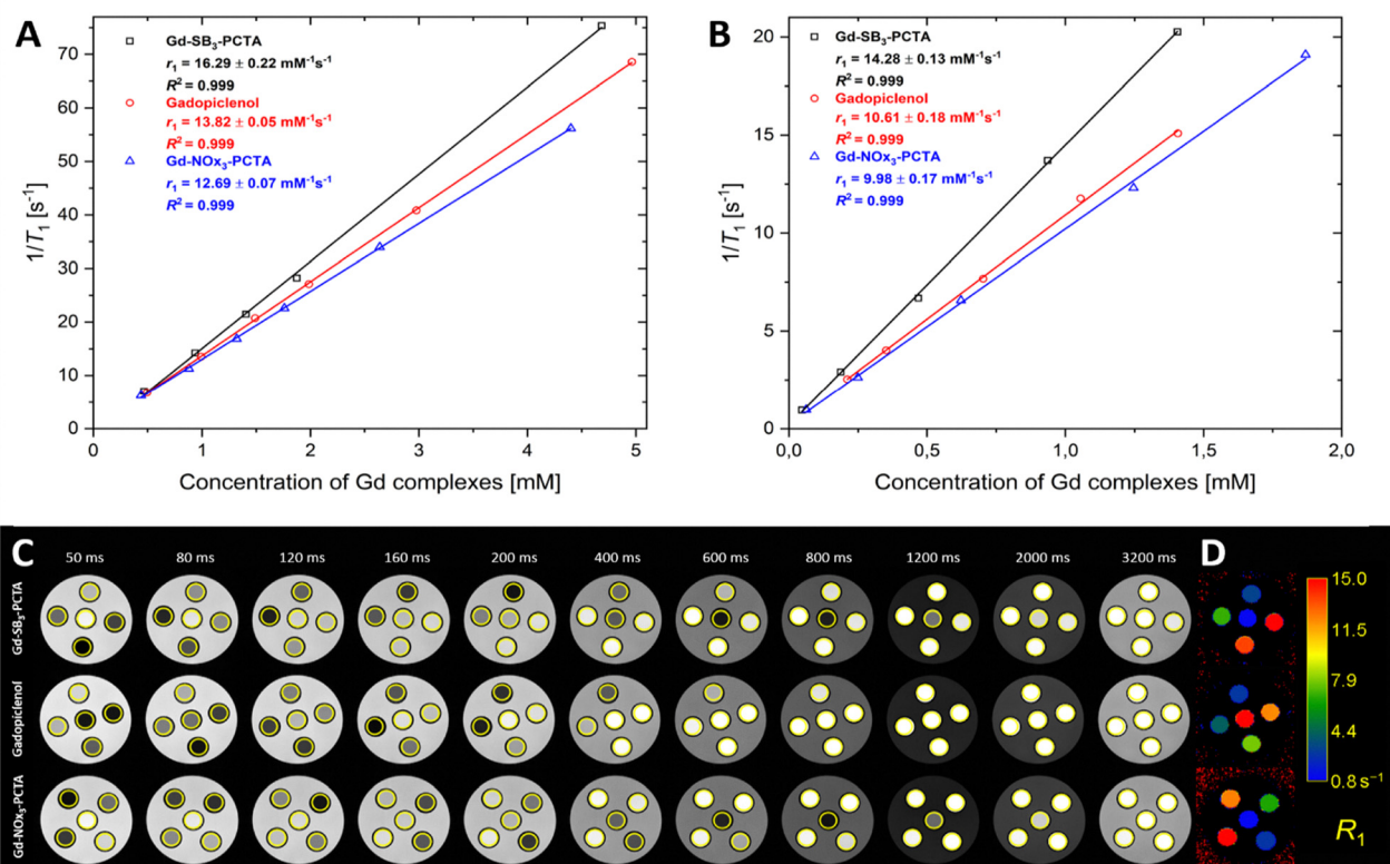
Fig. 3 (A) Longitudinal relaxivity ( r_1 ) determined from plotting the reciprocal relaxation time 1/T_1 versus the concentration of Gd-SB 3 -PCTA 11a , Gd-NOx 3 -PCTA 12a and gadopixelenol 3 in H 2 O at 37 °C and 1.4 T (60 MHz) (B) longitudinal relaxivity ( r_1 ) determined from plotting the reciprocal relaxation time 1/T_1 versus the concentration of Gd-SB 3 -PCTA 11a , Gd-NOx 3 -PCTA 12a and gadopixelenol 3 in H 2 O at room temperature and 7 T (300 MHz) (C) representative MR images acquired at 7 T at multiple inversion times (TI) ranging from 50 ms to 3200 ms of Gd-SB 3 -PCTA 11a , Gd-NOx 3 -PCTA 12a and gadopixelenol 3 in a phantom holder and surrounded by water. Yellow circles represent the regions of interest for five different concentrations of each compound used for subsequent quantitative analysis. (D) Color-coded R_1 relaxation rate map acquired at 7 T with an inversion-recovery spin-echo sequence with multiple inversion time delays for five different concentrations of each compound.
