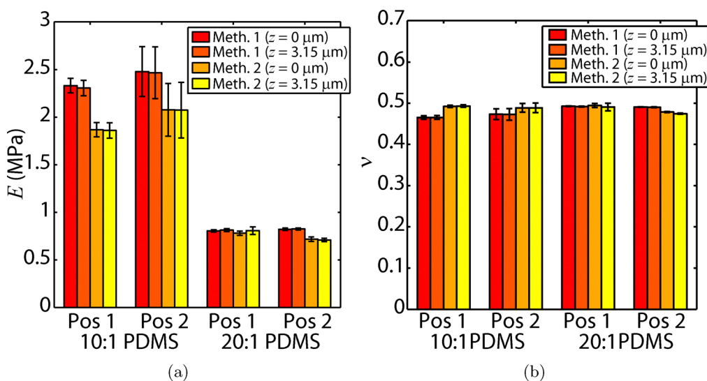
Fig. 9 Comparison of (a) E and (b) \nu calculated from the PT method (Method 1) and the hybrid method (Method 2) using displacements calculated from the FE model along the specimen surface and 3.15\ \mu\text{m} below the surface assuming perfectly bonded contact between the indenter and film. The height of each bar represents the corresponding mean, and each error bar represents the corresponding standard deviation.
