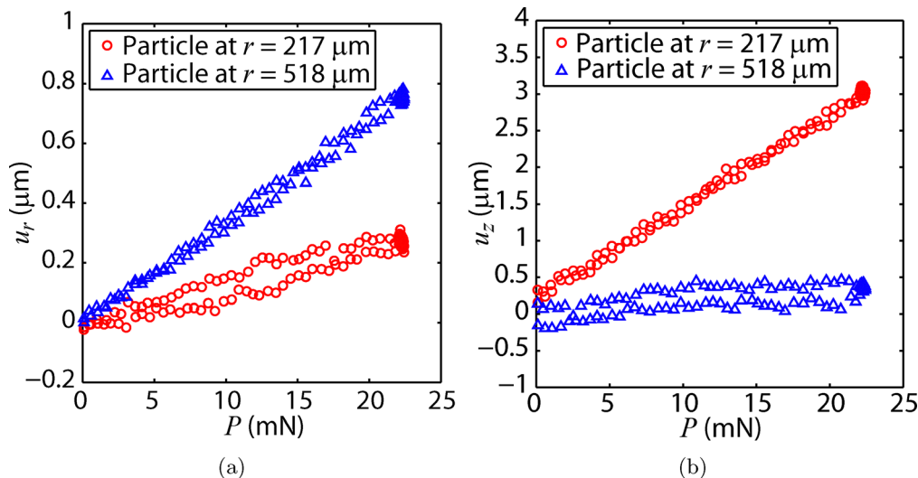
Fig. 8 (a) u_r and (b) u_z as a function of P for particles located 217\ \mu\text{m} and 518\ \mu\text{m} from the center of the indenter for a test on a 165\ \mu\text{m} thick 10 : 1 PDMS film on a glass substrate.
