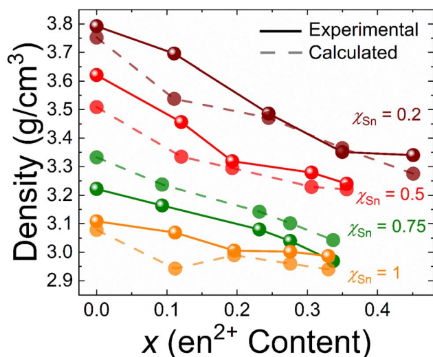
Fig. 4 Experimental and calculated density ( \text{g cm}^{-3} ) from single crystal refinements for each material plotted as a function of ethylenediammonium ( \text{en}^{2+} ) substitution. The experimental and calculated densities are represented by solid and dashed lines, respectively.
